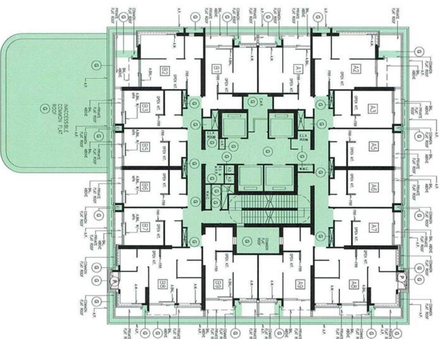
TOWER 1, 2ND FLOOR PLAN
